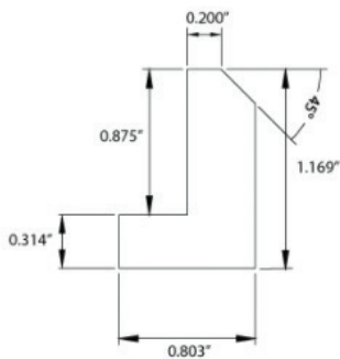
CHAMFER NOSING
